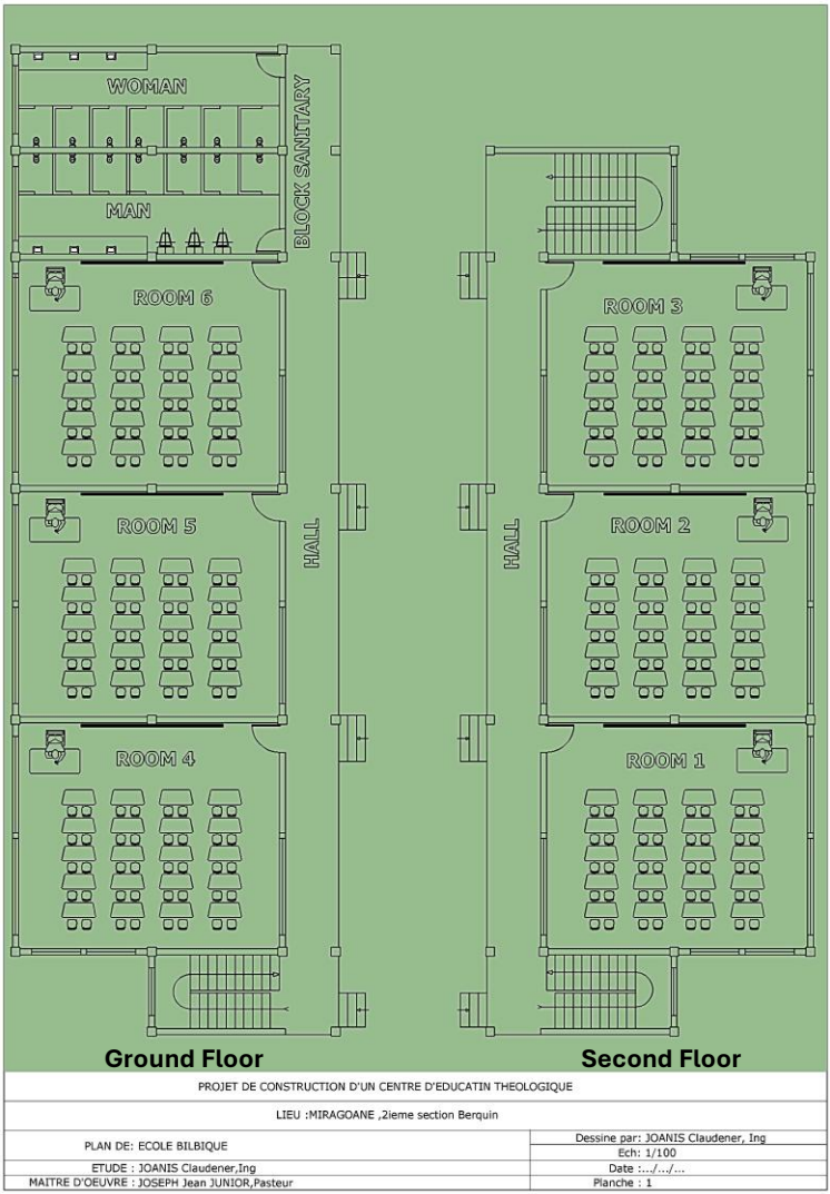
Classrooms (possible 2-story bldg.)
